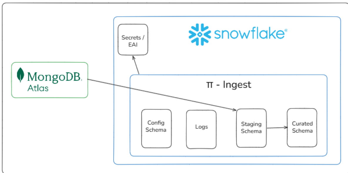
Fig. Pi-Ingest Architecture
